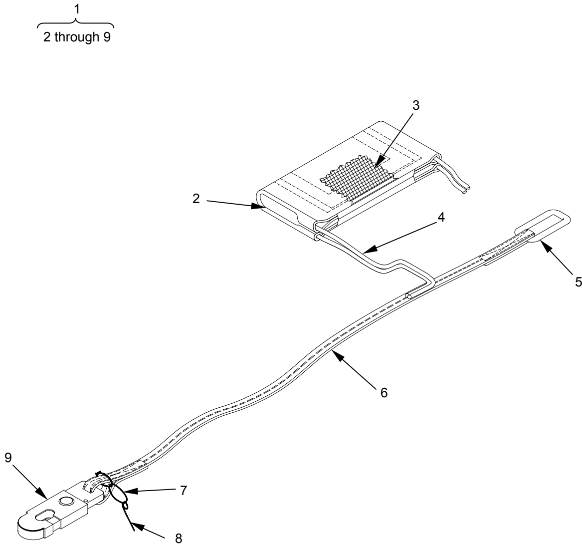
Fig 1. EXTENSION, STATIC LINE
