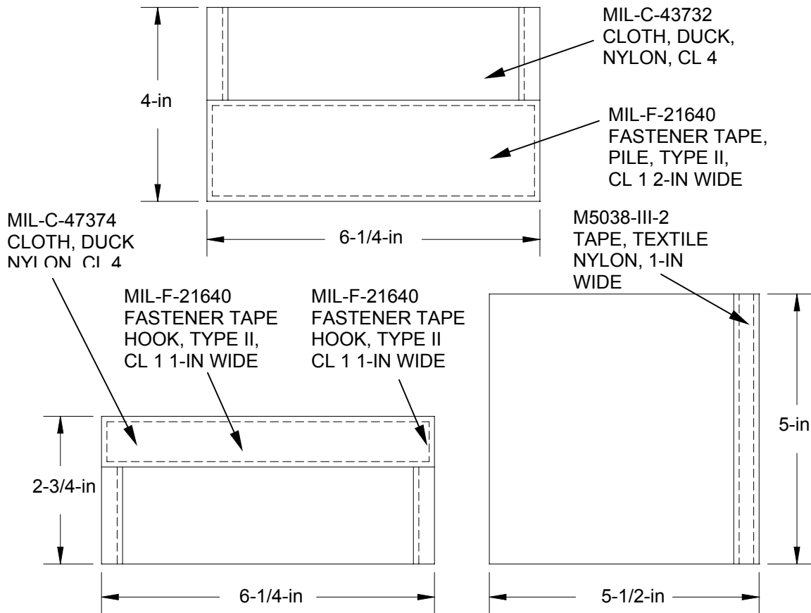
Fig. 22 (CONTAINER FRONT MOUNTED) LOWERING LINE POCKET, FLAPS AND LOOP
