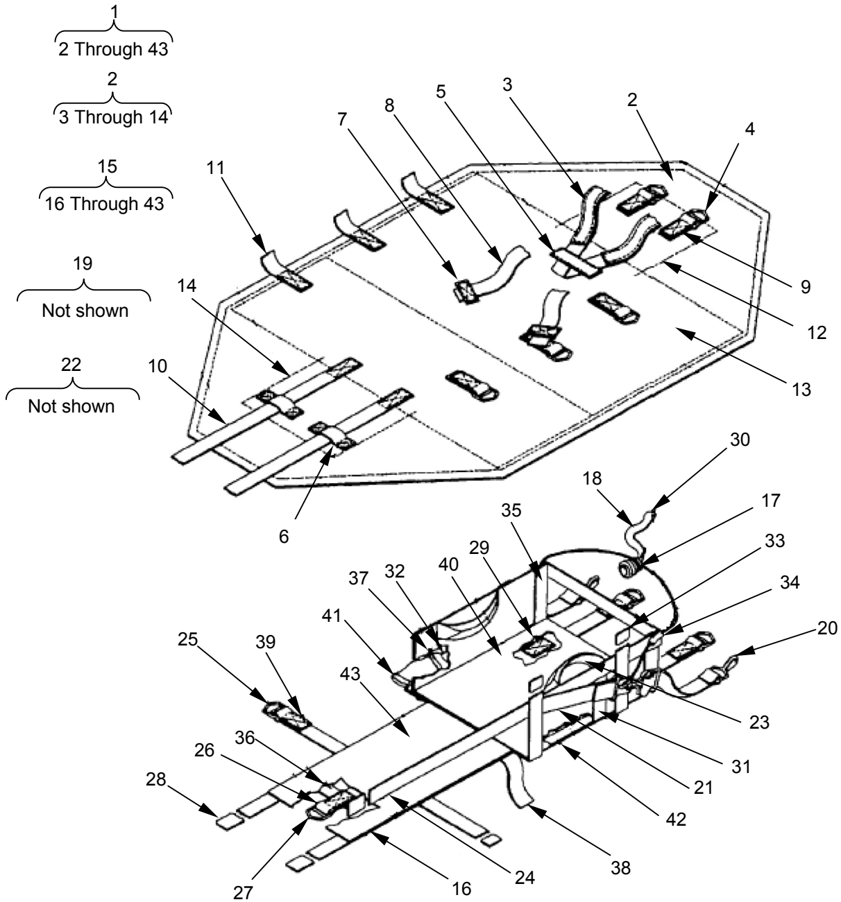
Fig 9. PARACHUTIST'S WEAPONS AND INDIVIDUAL EQUIPMENT PACK AND HARNESS ASSEMBLY
