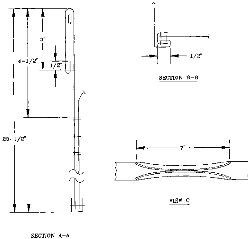
Fig. 24 (CONTAINER FRONT MOUNTED) KIT, BAG ASSEMBLY (SHEET 2 OF 2)
