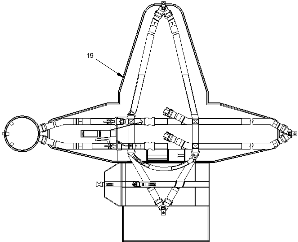
CONTAINER, FRONT MOUNT (AIRPAC)
