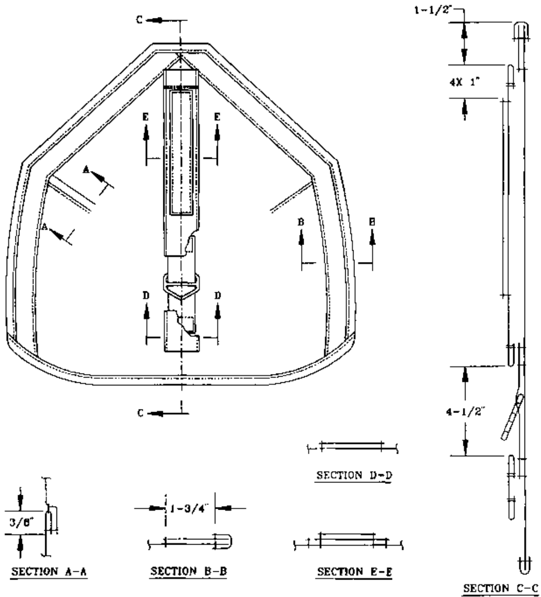
Fig. 28 (CONTAINER SIDE MOUNTED) UPPER CAP ASSEMBLY (SHEET 2 OF 2)
