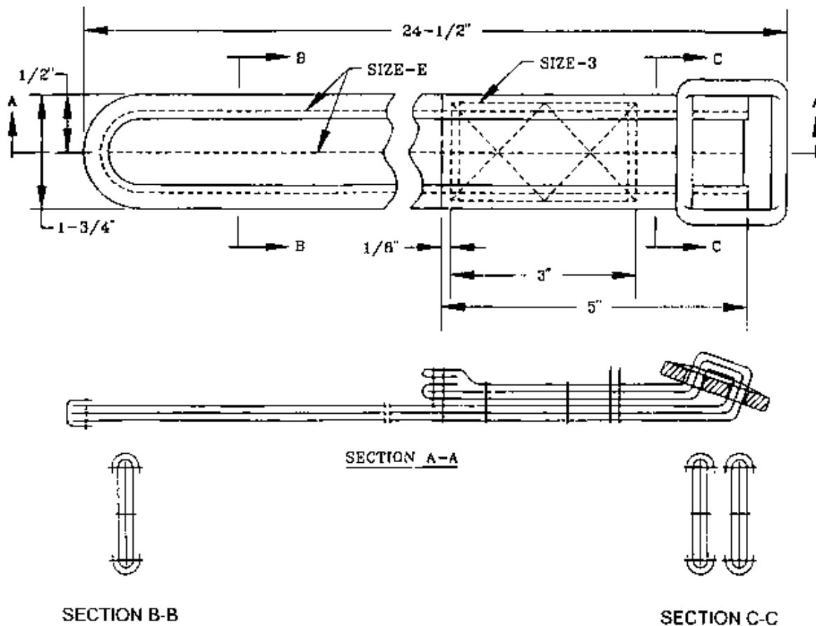
Fig. 4 (ACCESSORY SET, SCUBA) STRAP, WAISTBAND EXTENSION
