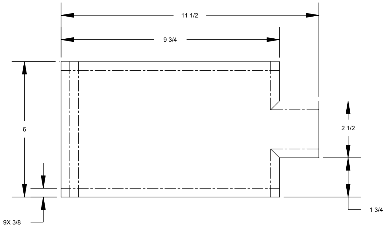
Fig. 11 (INDIVIDUAL WEAPONS CASE, M-1950 (NYLON)) POCKET ASSEMBLY, LOWERING
