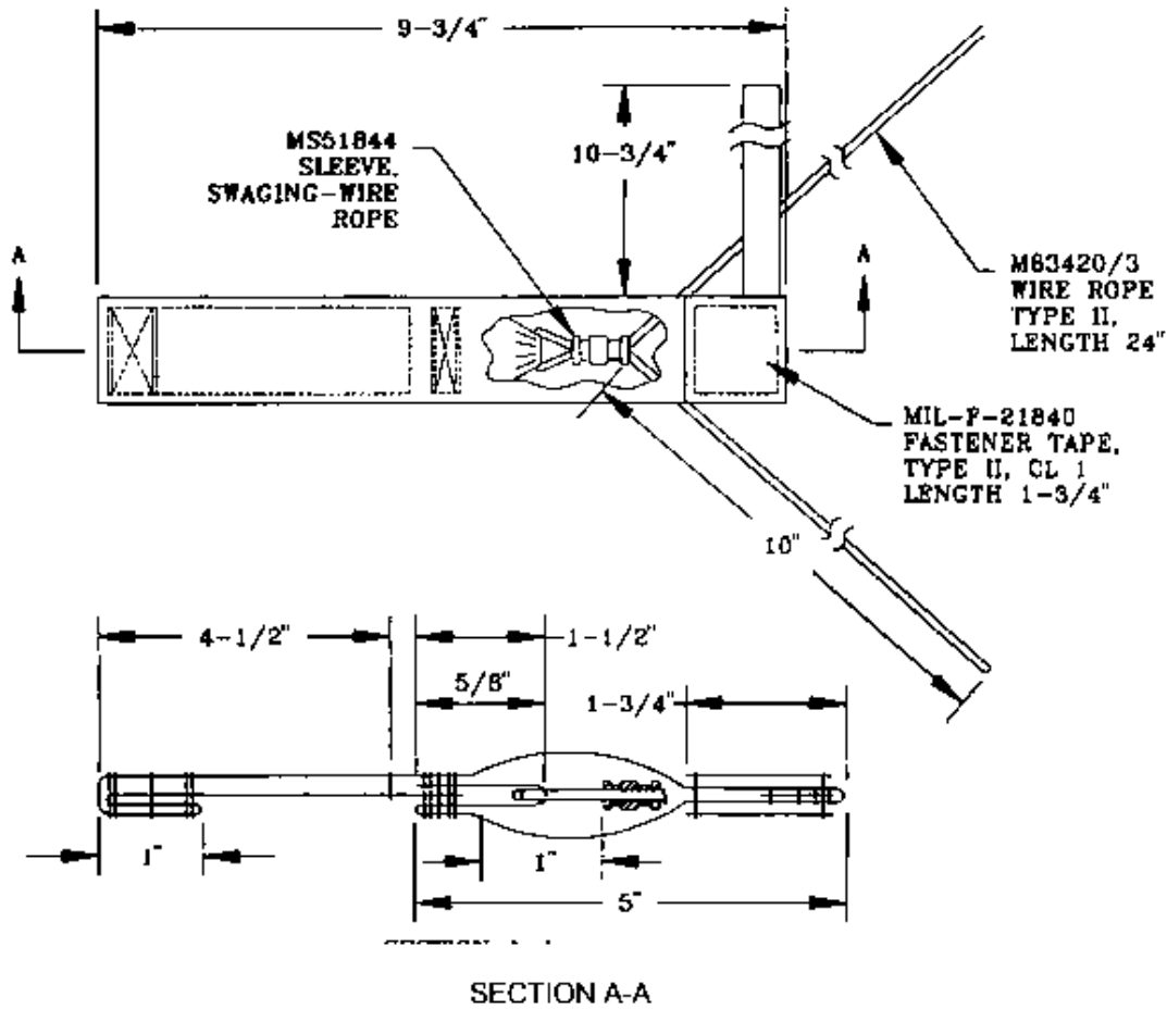
Fig. 27 (CONTAINER FRONT MOUNTED) RELEASE HANDLE ASSEMBLY
