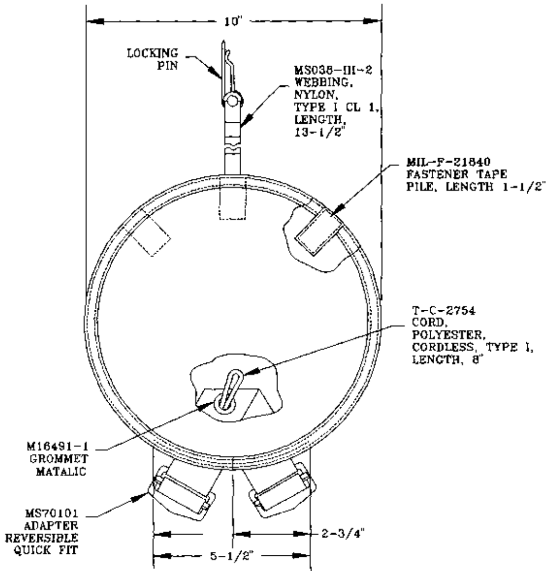
Fig. 21 (CONTAINER FRONT MOUNTED) CLOSING FLAP ASSEMBLY
