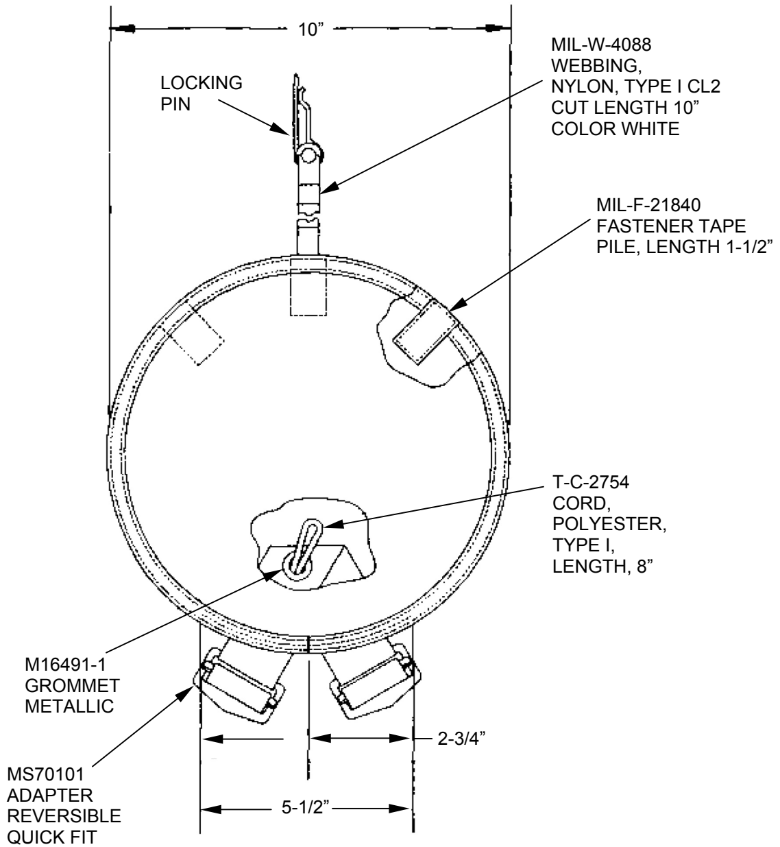
Fig. 20 (CONTAINER FRONT MOUNTED) VERTICAL RESTRAINT ASSEMBLY (SHEET 2 OF 3)
