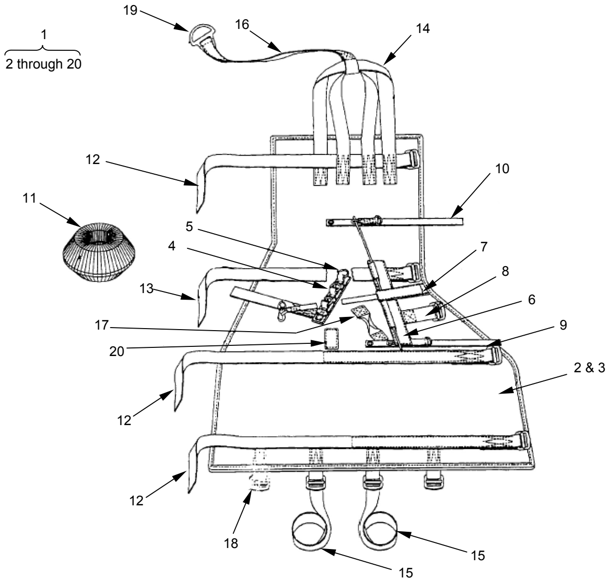
Fig 10. JUMP PACK, STINGER MISSILE
