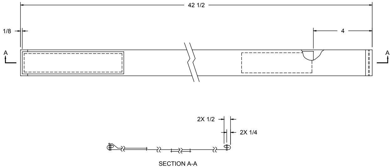
Fig. 13 (INDIVIDUAL WEAPONS CASE, M-1950 (NYLON)) LOWER LEG STRAP ASSEMBLY
