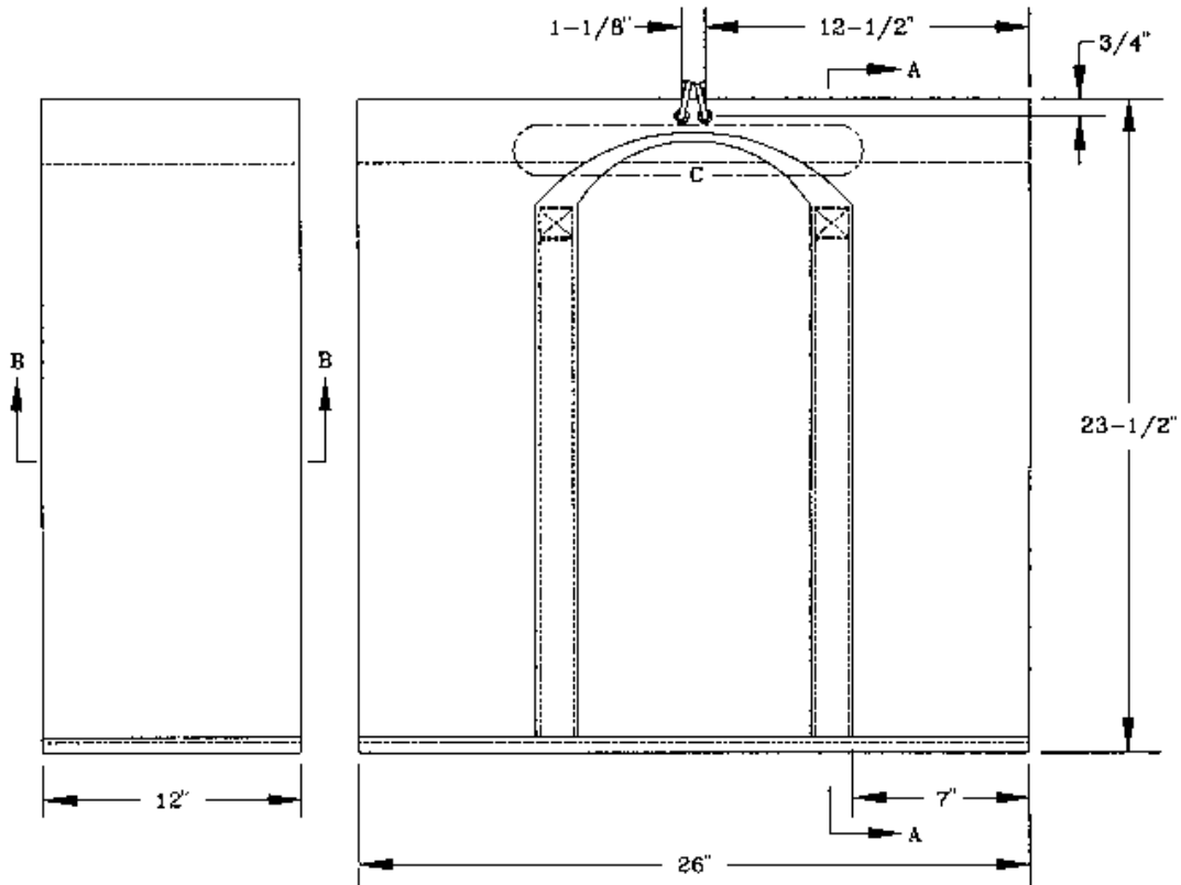
Fig. 24 (CONTAINER FRONT MOUNTED) KIT, BAG ASSEMBLY (SHEET 1 OF 2)
