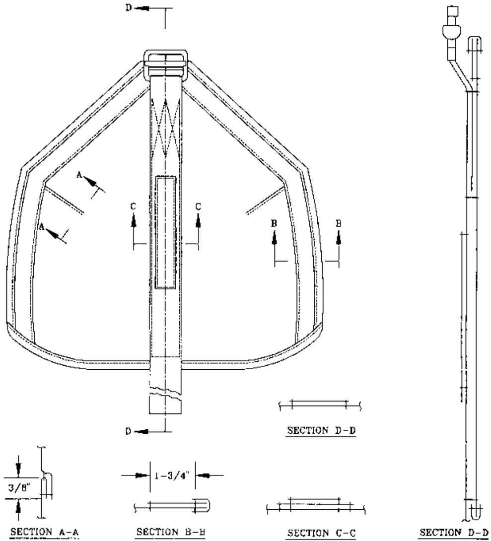
Fig. 29 (CONTAINER SIDE MOUNTED) LOWER CAP ASSEMBLY (SHEET 2 OF 2)
