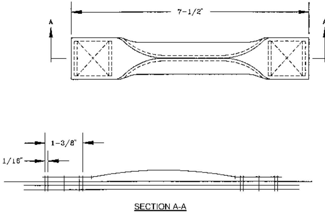
Fig. 17 (STINGER MISSILE PACK) STRAP, CARRYING
