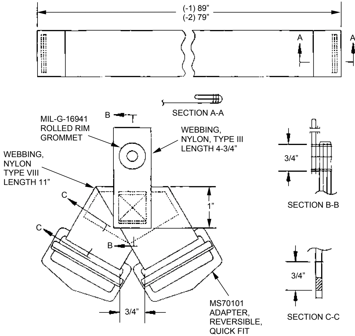
Fig. 20 (CONTAINER FRONT MOUNTED) VERTICAL RESTRAINT ASSEMBLY (SHEET 3 OF 3)
