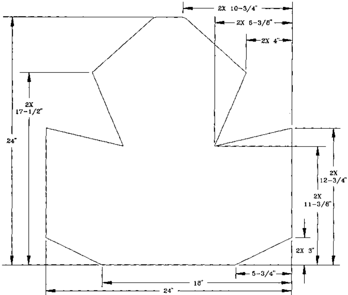
Fig. 29 (CONTAINER SIDE MOUNTED) LOWER CAP ASSEMBLY (SHEET 1 OF 2)
