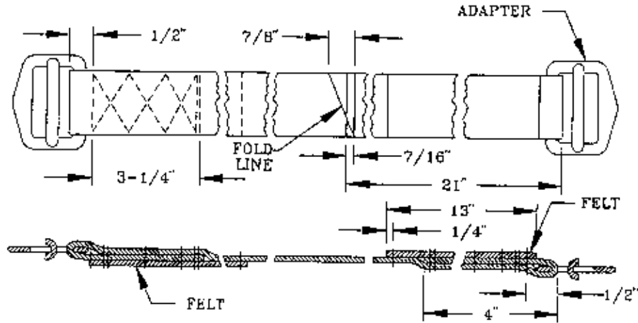
Fig. 14 (EQUIPMENT PACK AND HARNESS ASSEMBLY) UPPER SUSPENSION STRAP
