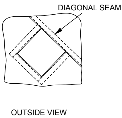
(A) RECTANGULAR PATCH INCLUDING A DIAGONAL SEAM
