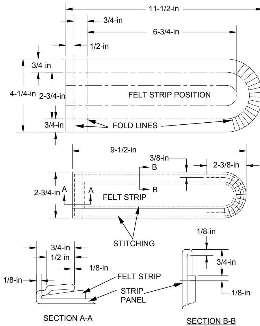
Fig. 10 (INDIVIDUAL WEAPONS CASE (COTTON)) M-1950, STRIP PANEL
