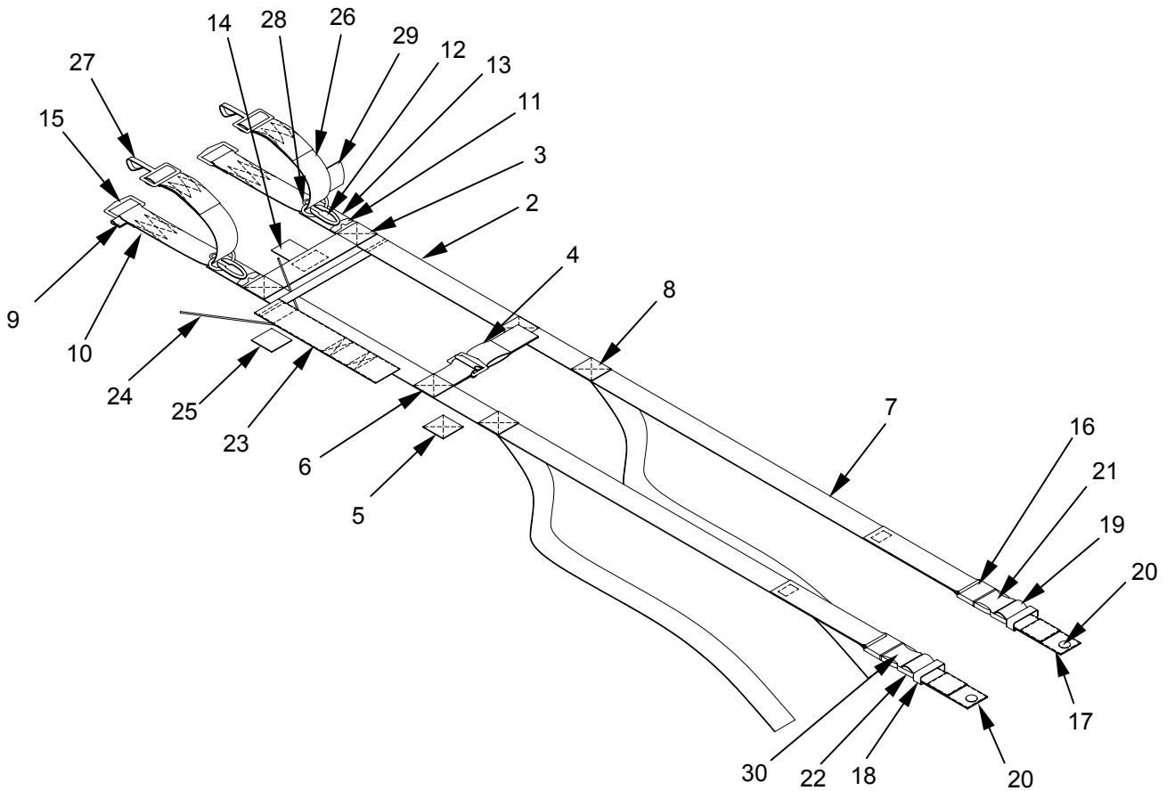
Fig 5. HARNESS, SINGLE POINT RELEASE
