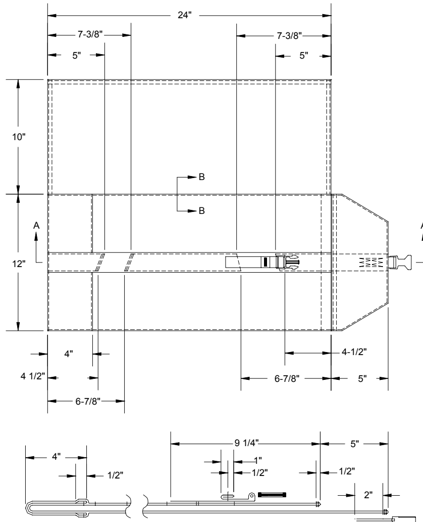
Fig. 23 (CONTAINER FRONT MOUNTED) SIDE CONTAINER ASSEMBLY
