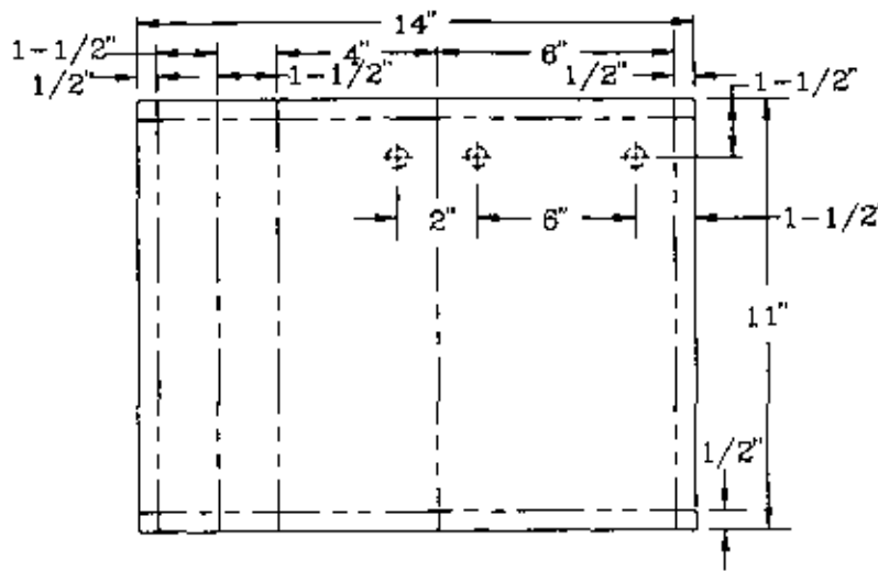
Fig. 9 (INDIVIDUAL WEAPONS CASE, M-1950 (COTTON)) POCKET ASSEMBLY, LOWERING
