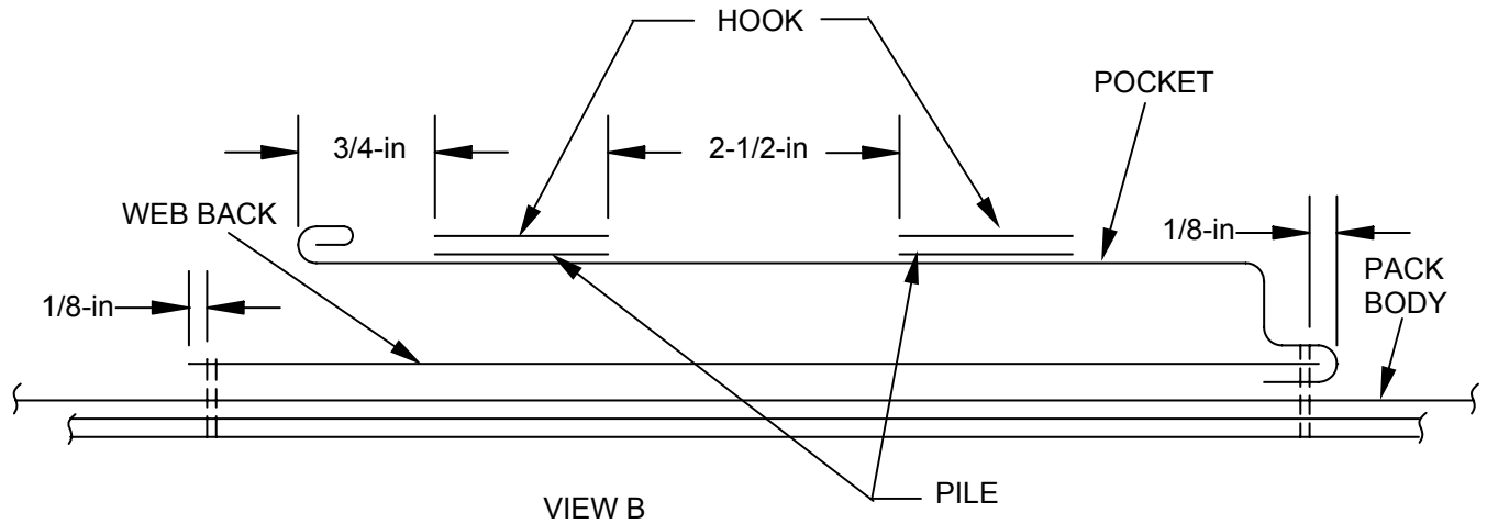
Fig. 7 (AT4 PACK) POCKET ASSEMBLY LOWERING LINE (SHEET 2 OF 2)
