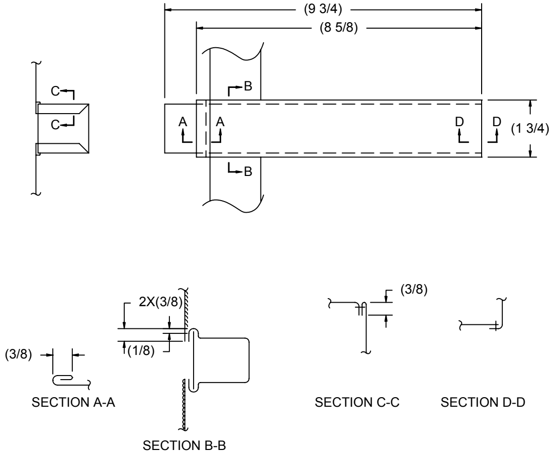
Fig. 12 (INDIVIDUAL WEAPONS CASE, M-1950 (NYLON)) LOWER STRAP POCKET ASSEMBLY
