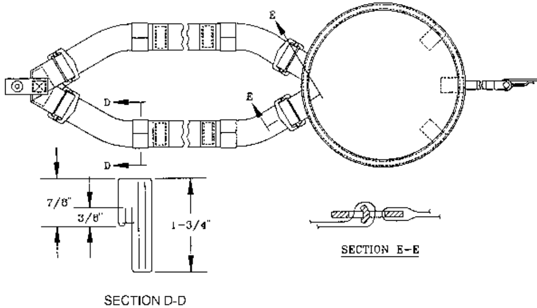
Fig. 20 (CONTAINER FRONT MOUNTED) VERTICAL RESTRAINT ASSEMBLY (SHEET 1 OF 3)
